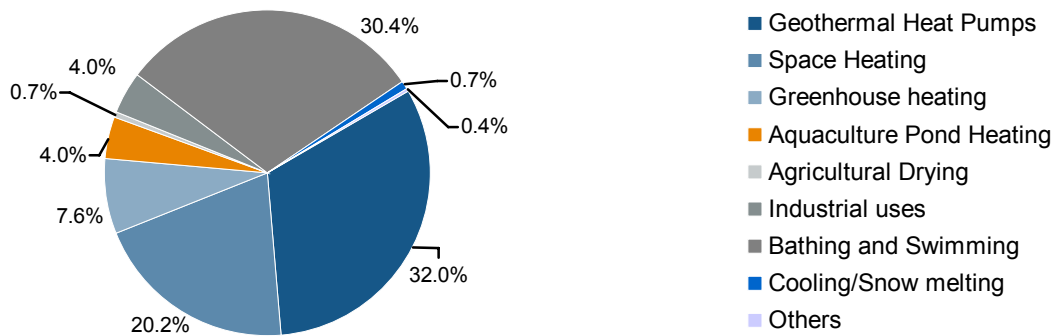
Figure 11-7 Direct applications of geothermal worldwide
