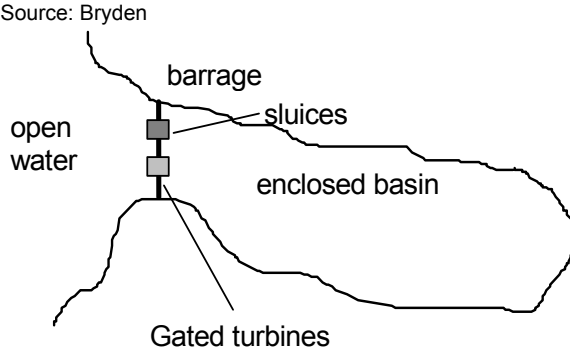
Figure 13-2 Hypothetical tidal barrage configuration Source: Bryden
