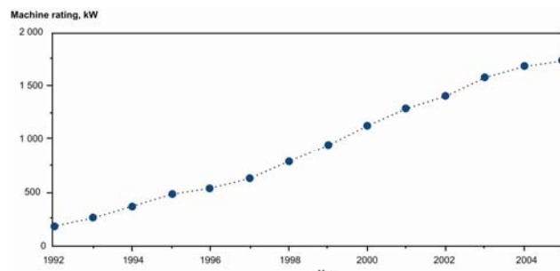
Figure 12-3 Average size of wind turbines installed in Germany, 1992-2005
