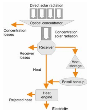
Figure 10-12 Flow diagram for a typical solar thermal power plant
