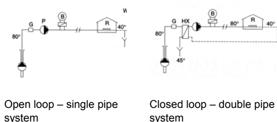
Figure 11-8 Two main types of district heating system
