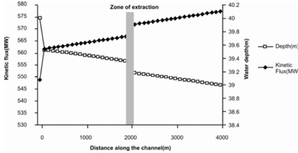
Figure 13-11 Influence of artificial energy extraction on the water depth and the kinetic energy flux
