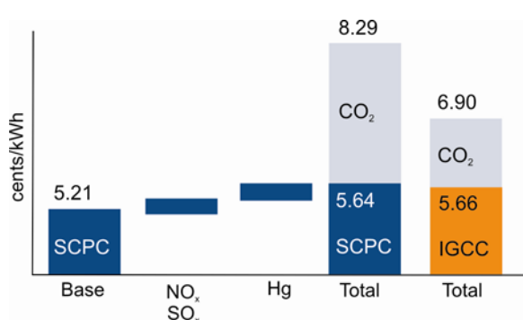
Figure 1-4 Cost of electricity comparison
