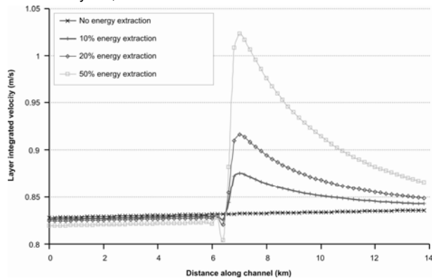
Figure 13-14 Predicted flow disruption close to the sea bed
