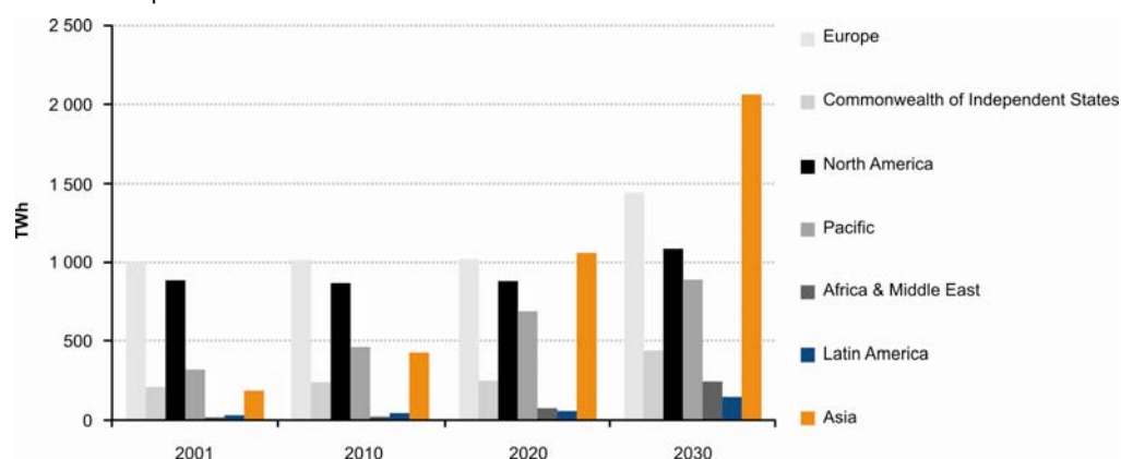
Figure 6-17 Electricity generation from nuclear power in the WETO-H 2 reference case
