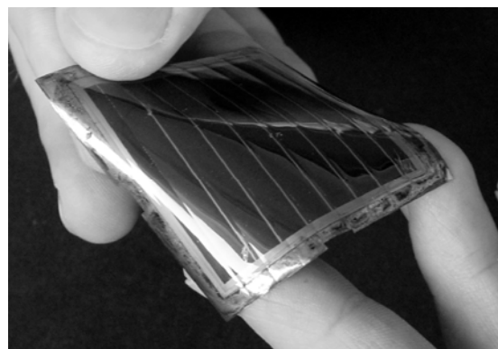
Figure 10-11 Flexible monolithic CIGS prototype mini-module on a polymer foil
