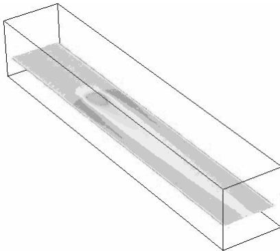
Figure 13-13 Numerical model of flow in the immediate vicinity of a tidal current device
